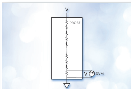
Figure 2. A high voltage divider is typically used to measure voltages above the instrument's direct input range.
