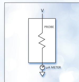
Figure 4. Vitrek's 4700 meter measures microamperes using high voltage SmartProbes.
